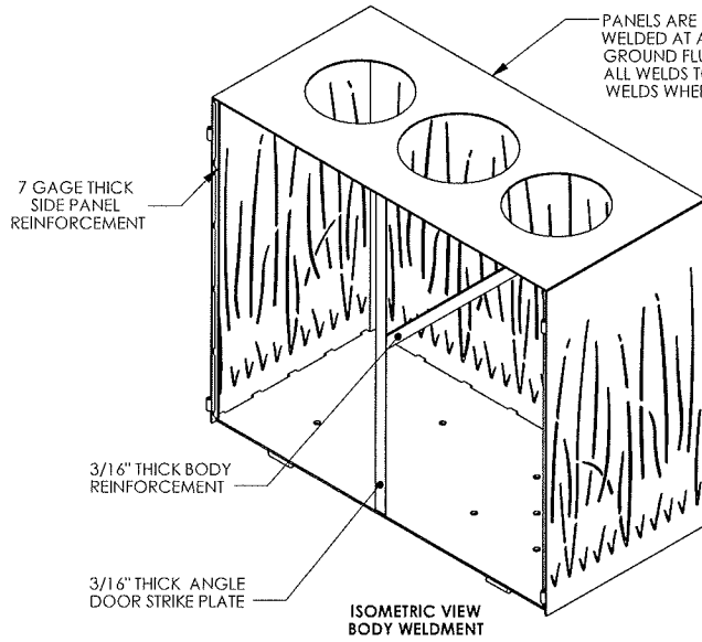
ISOMETRIC VIEW BODY WELDMENT
